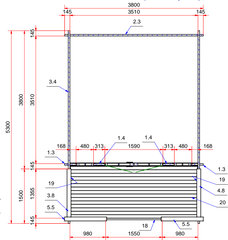
Plan huschen (house plan)
