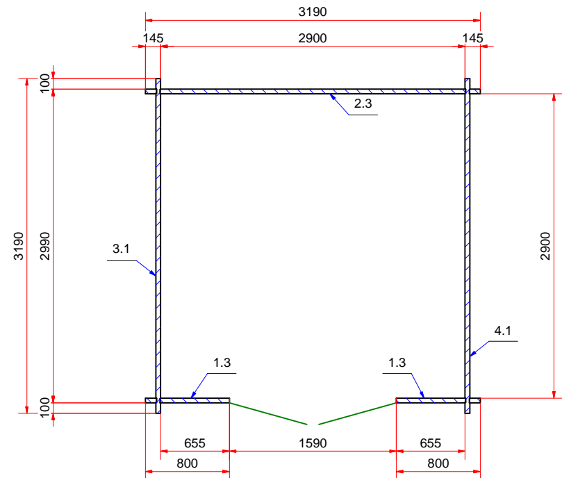
Plan huschen (house plan)
