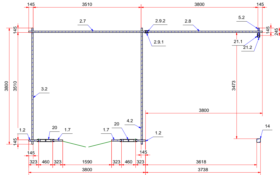
Plan huschen (house plan)
