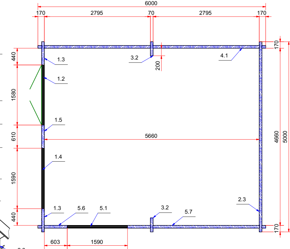
Plan huschen (house plan)
