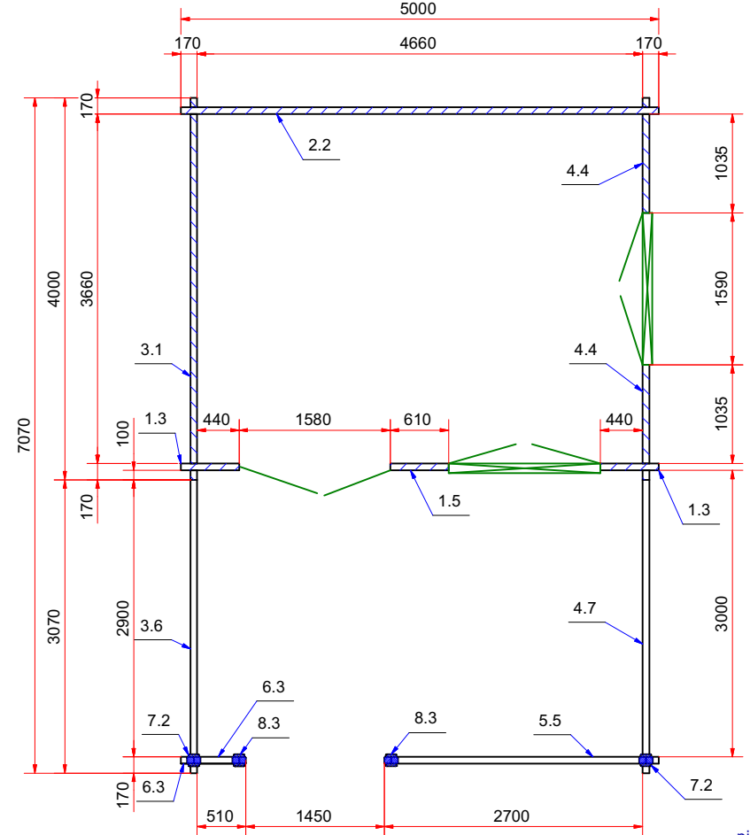
Plan huschen (house plan)
